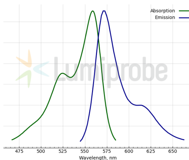
Cyanine3B absorption and emission spectra
