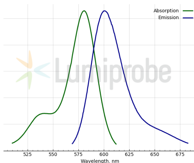
Absorption and emission spectra of Mito Red CMXRos
